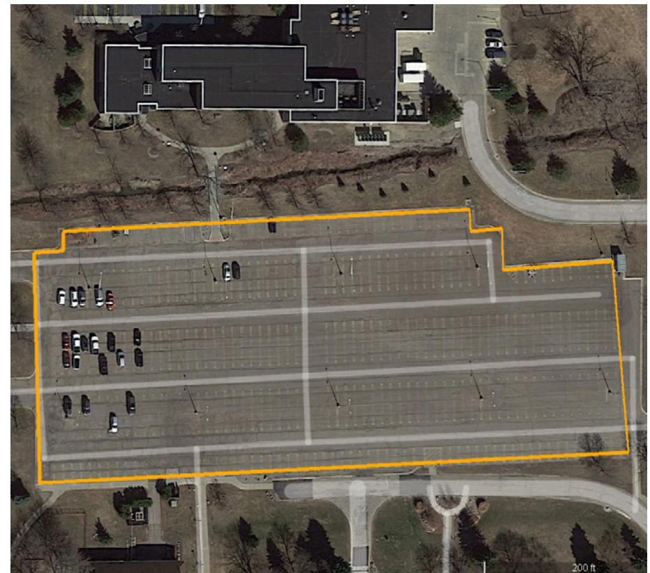
Figure 6. Public Parking Lot Proposed Solar Area
