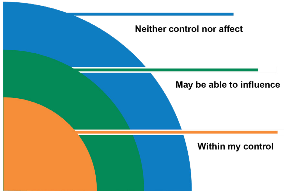
Figure 28. Influence Model
